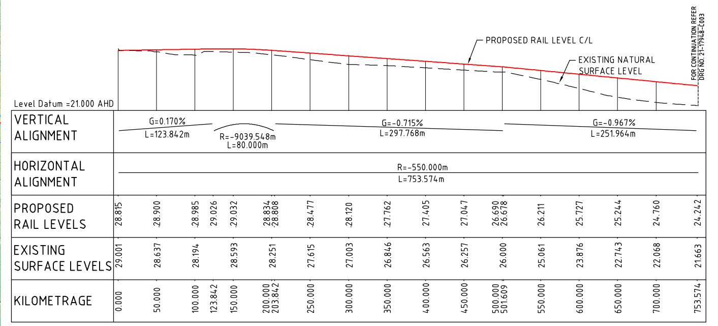
PROFILE PROPOSED NORTH CONNECTION TRACK C/L SCALE 1:2500 HORIZONTAL 1:250 VERTICAL
