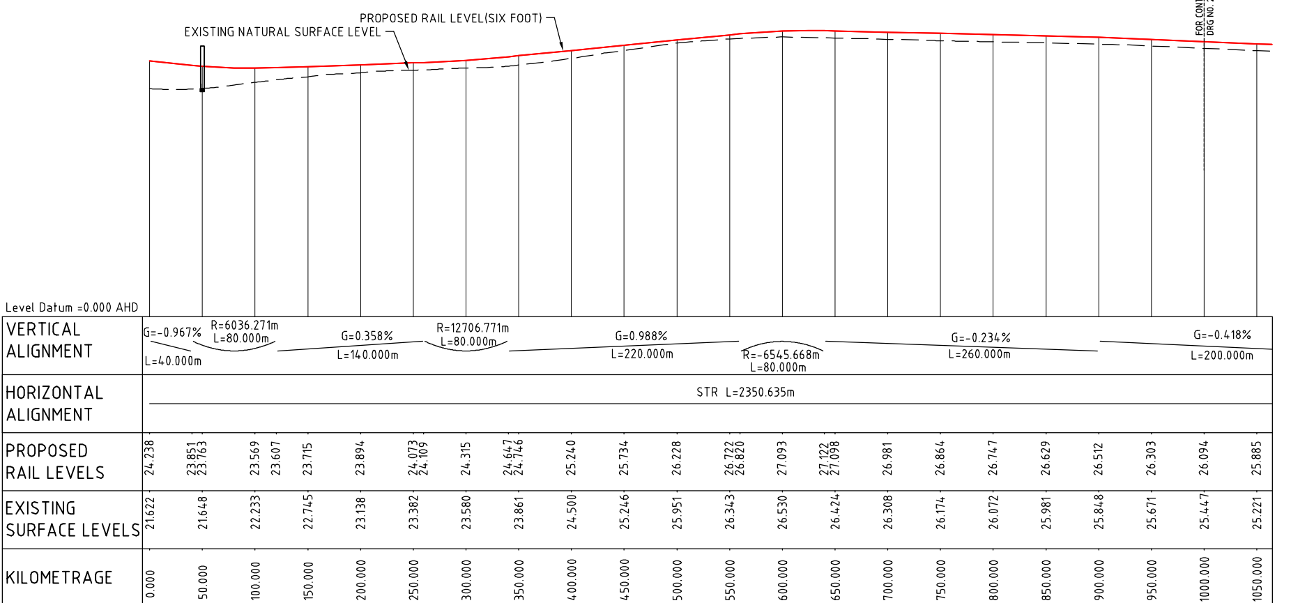
PROFILE PROPOSED SIX FOOT ALIGNMENT SCALE 1:2500 HORIZONTAL 1:250 VERTICAL
