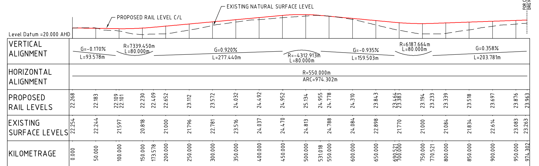
PROFILE PROPOSED SOUTH CONNECTION TRACK C/L SCALE 1:2500 HORIZONTAL 1:250 VERTICAL
